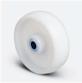
Wheel: ZMZ Polyamide wheel (natural white), without threadguards, roller bearing, -20°C to +80°C
